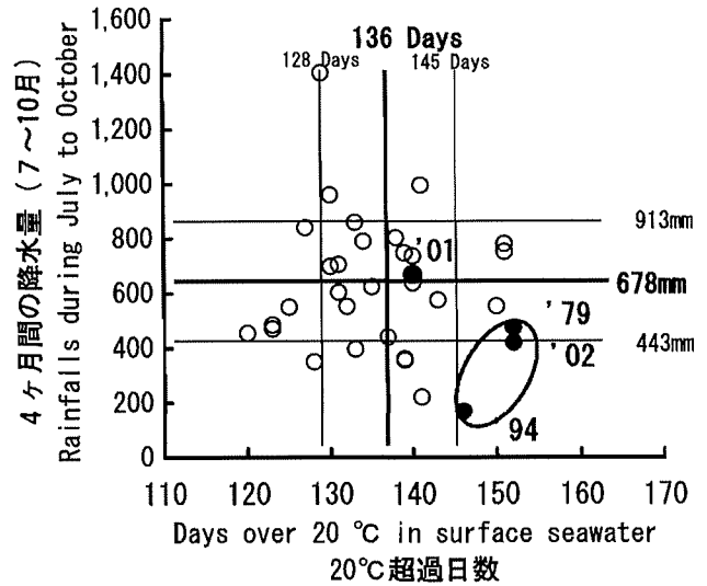
図3 大量へい死発生年と水温20℃超過日数および7～10月の4ヶ月間降水量との関係 Fig. 3 Relationship between rainfalls during July to October and days over 20°C in seawater surface layer at HPFMTC. Closed circles represent the year when mass mortality occurred in oyster culture.
