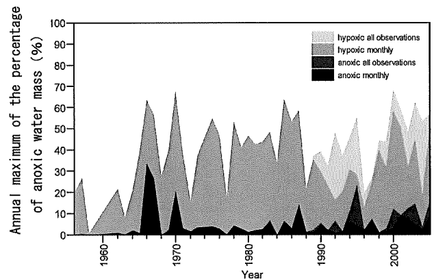
Figure 5. Change of annual maximum of the percentage of hypoxic ( 2.5 \text{ ml} \cdot \text{l}^{-1} , gray and light gray) and anoxic ( 0.5 \text{ ml} \cdot \text{l}^{-1} , black and dark gray) water mass in the vertical cross section in Tokyo Bay. Gray and black show the results from monthly fixed observation only while light gray dark and gray for data since 1989 show all observations for each year.
