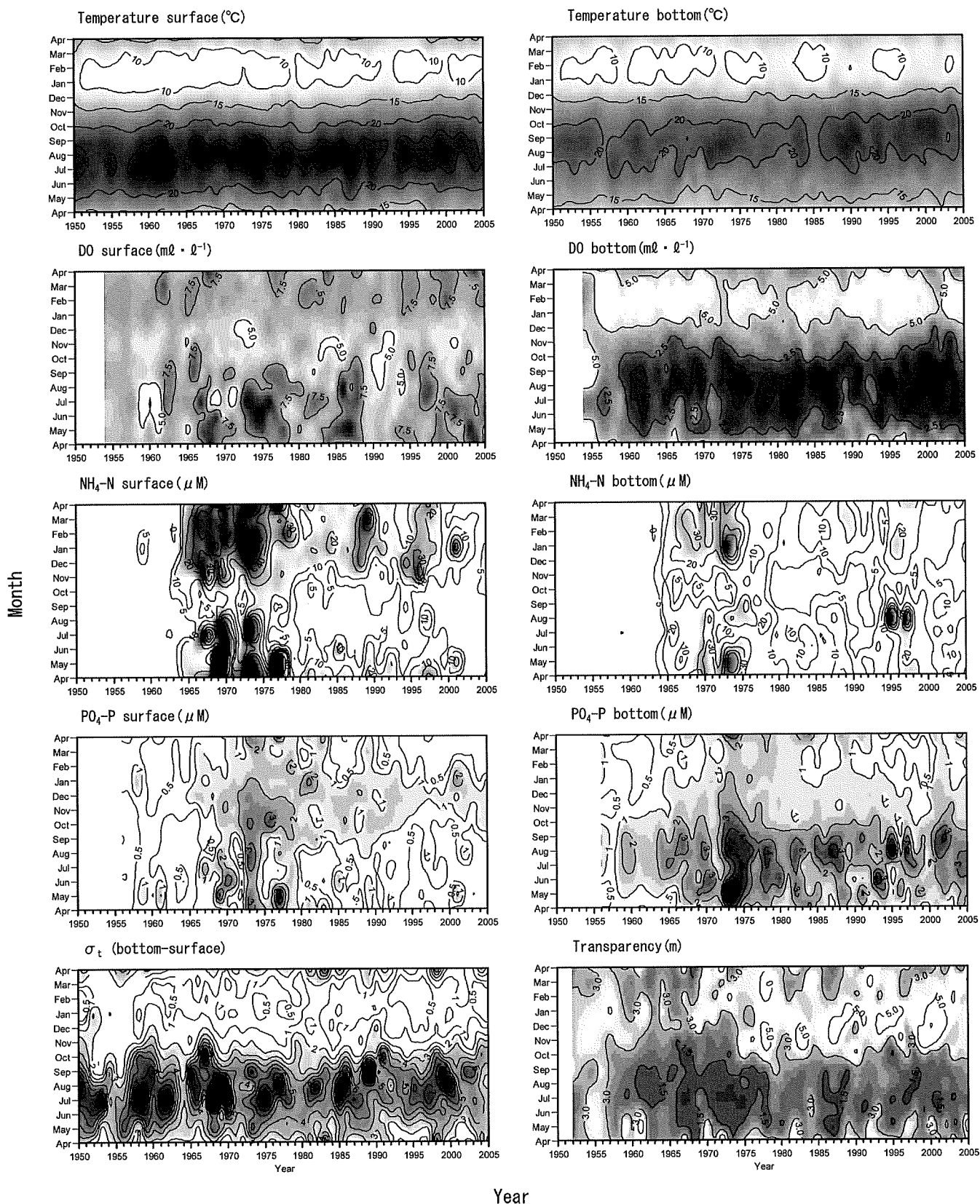
Figure 2. Temporal fluctuations of water temperature ( ^{\circ}\text{C} ), DO ( \text{mL} \cdot \text{L}^{-1} ), \text{NH}_4\text{-N} ( \mu\text{M} ), \text{PO}_4\text{-P} ( \mu\text{M} ), \sigma_t (bottom-surface) and transparency (m) at Stn. 3. X-axis is for year; Y-axis for month.
