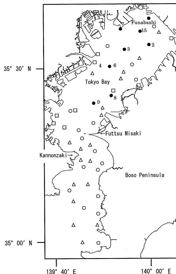
Figure 1. Observational stations in Tokyo Bay. Marine observations in Tokyo Bay by CPFRC were started at 1948. There have been six large alternations of the stations, and 26 are active at present. Data from six stations (15, 2, 3, 6, 8, 9; solid circles), which have been active since 1948, were mainly used for this analysis. Open circles were from an intermediate year to date. Open squares were from initial to the way. Open triangles are stations that were active from 1966 until 2001.
