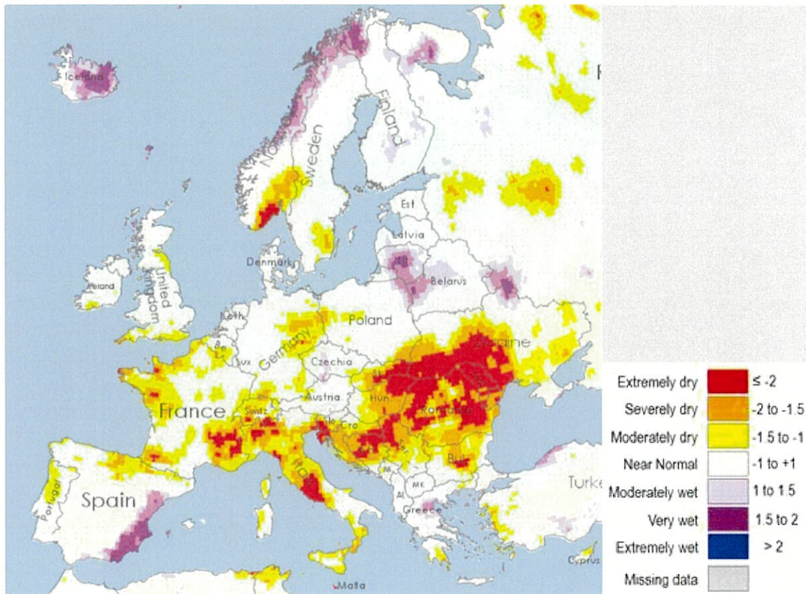
Figure 3: Standardized Precipitation Index SPI-6, February-July 2022.
