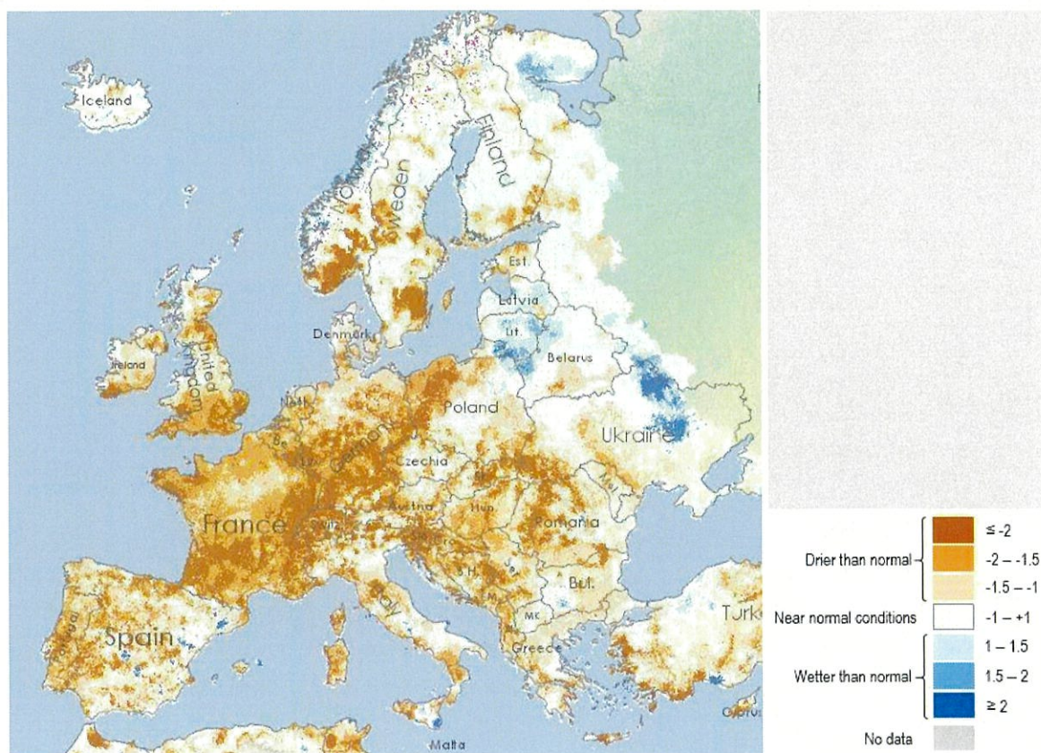
Figure 4: Soil Moisture Anomaly – beginning of August 2022.
