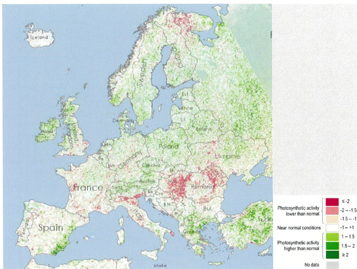
Figure 5: fAPAR anomaly - beginning of August 2022.
